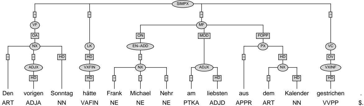
Figure 3: A sample tree from Tüba-D/Z.
